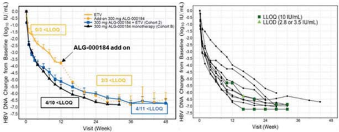
Figure 8 – DNA over time in HBeAg positive subjects dosed with ALG-000184 with or without ETV or ETV alone (Yuen et al., AASLD 2023)
